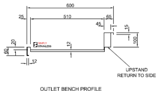
OUTLET BENCH PROFILE
